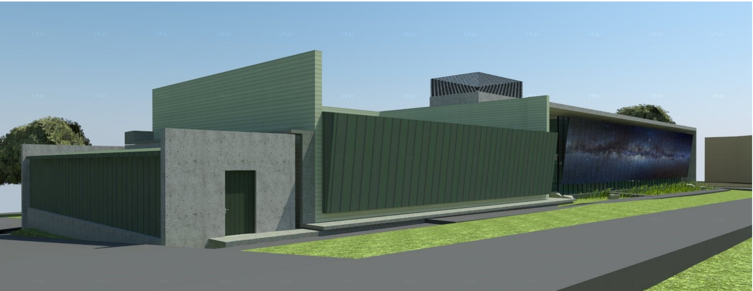
North (front) Façade of New Office Building (right), Data Center and Electrical Building (left)
